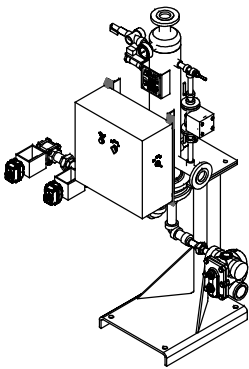
ISOMETRIC VIEW
