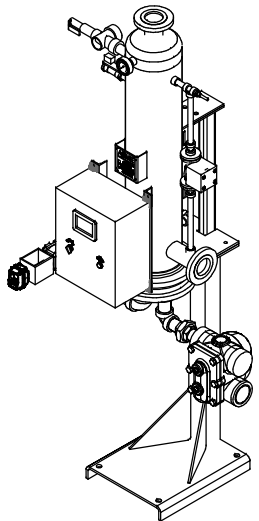
ISOMETRIC VIEW
