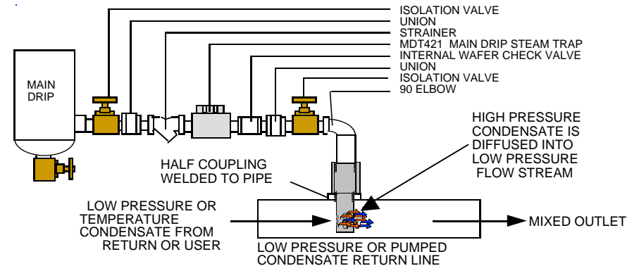
TYPICAL HOOKUP
