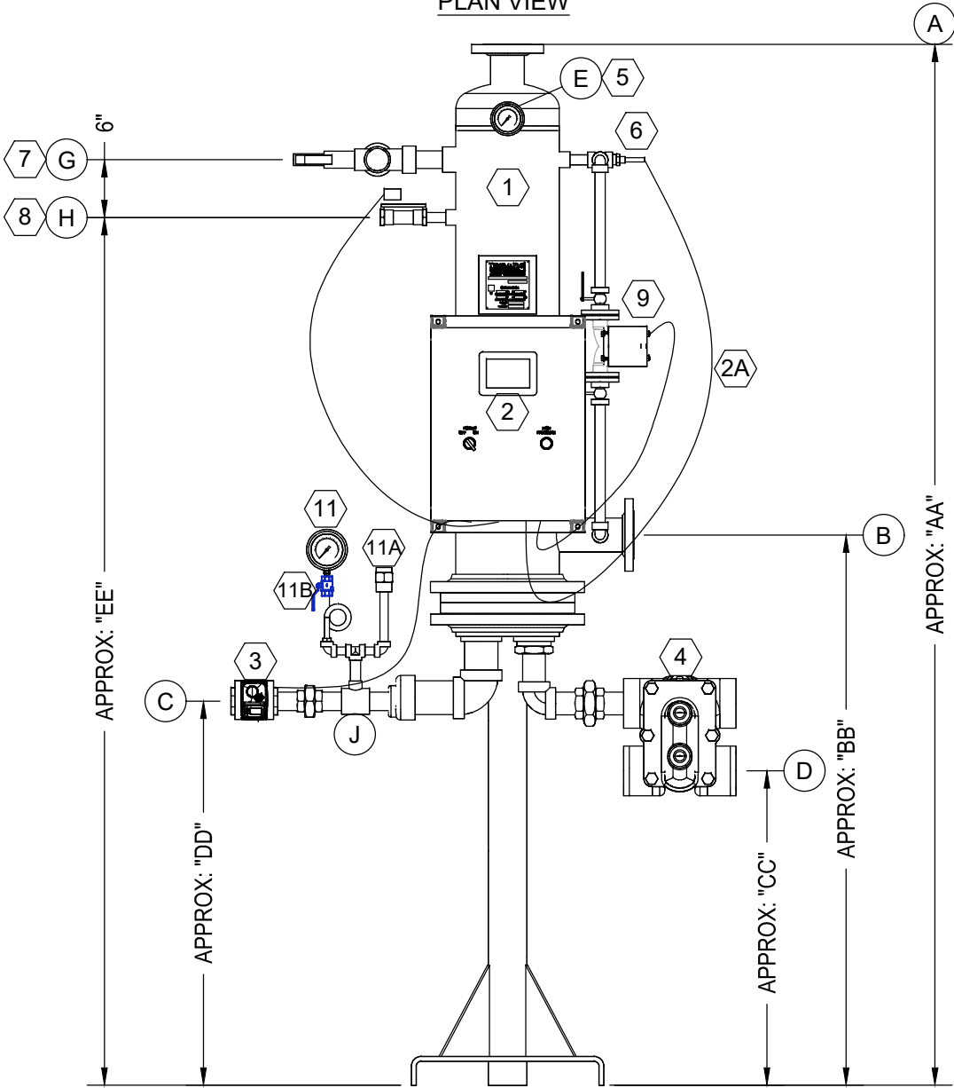
FRONT VIEW
