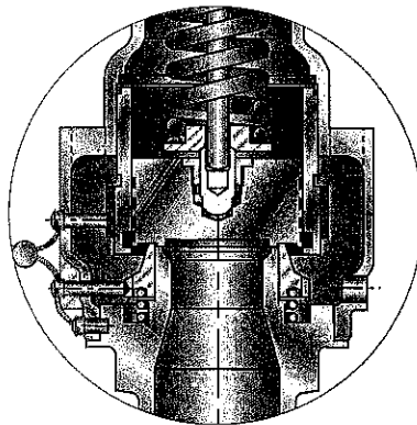
Models 6182, 6121, 6130, 6186 Top Outlet Configuration
