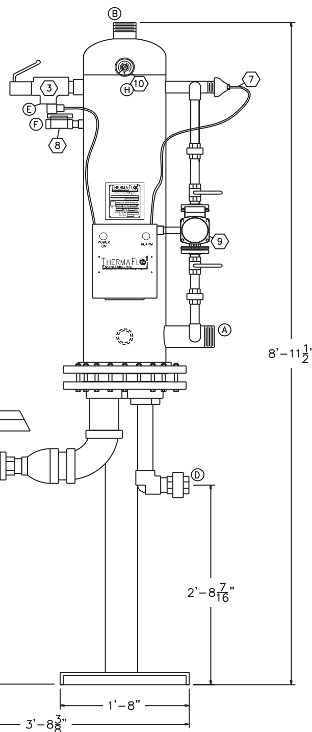
ELEVATION VIEW
