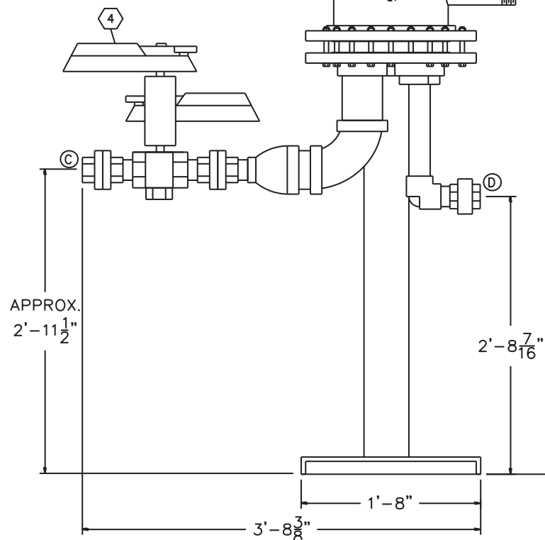
ELEVATION VIEW
